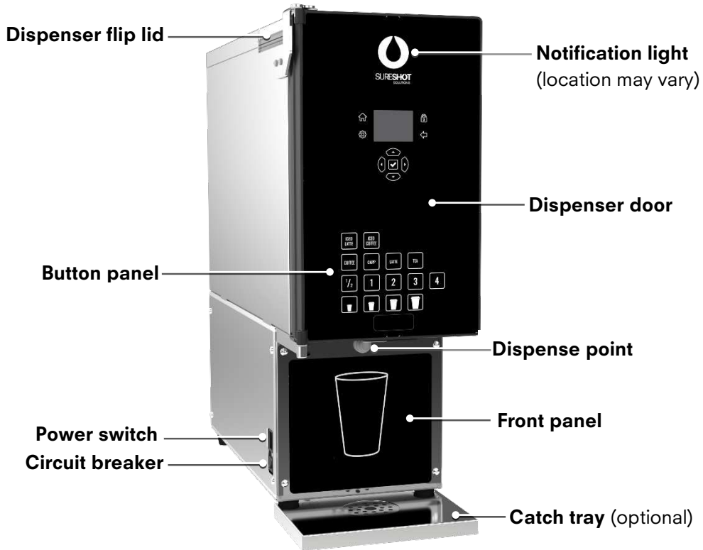
Figure 1: Main exterior components of model AC110-V2 (Product Tank)
