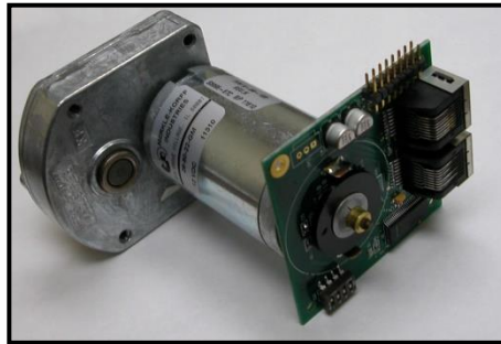
Motor coupler assembly
